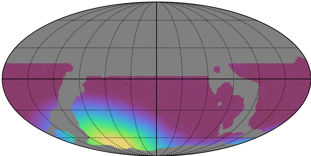
weather_cloudso10v3.4_10yrs WFD all bands: Min moonDistance
