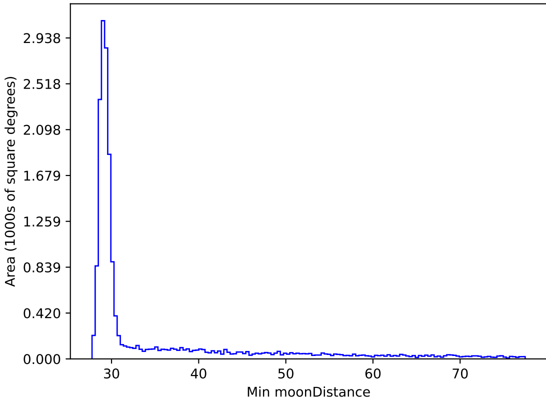
weather_cloudso10v3.4_10yrs WFD all bands: Min moonDistance
