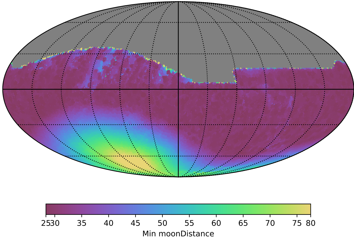
weather_cloudso10v3.4_10yrs All sky z band: Min moonDistance
