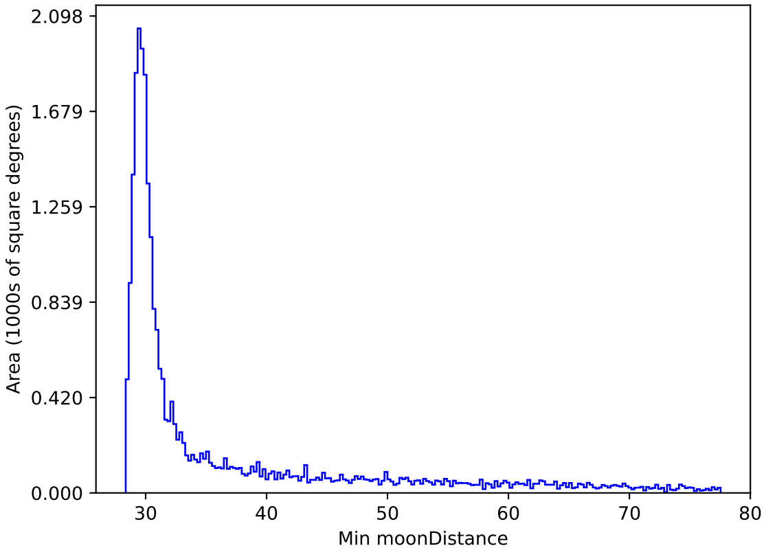
weather_cloudso10v3.4_10yrs All sky z band: Min moonDistance
