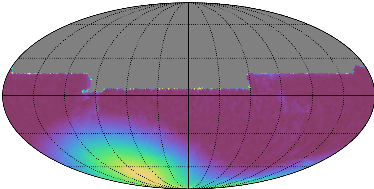
weather_cloudso10v3.4_10yrs All sky y band: Min moonDistance
