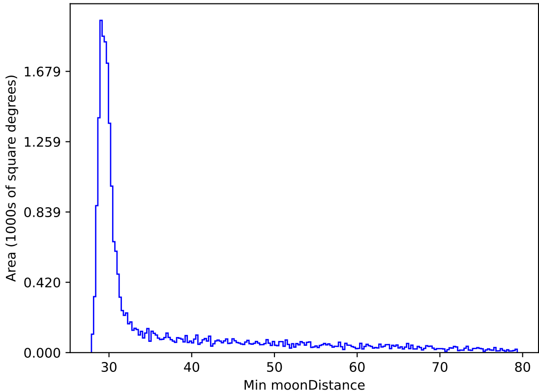
weather_cloudso10v3.4_10yrs All sky y band: Min moonDistance
