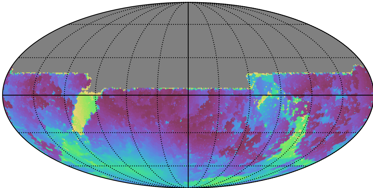
weather_cloudso10v3.4_10yrs All sky u band: Min moonDistance
