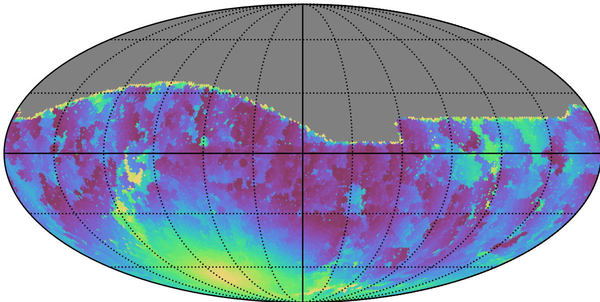
weather_cloudso10v3.4_10yrs All sky g band: Min moonDistance
