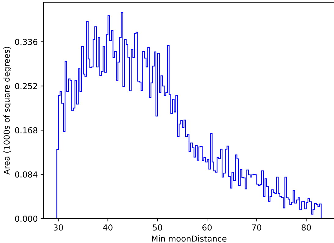
weather_cloudso10v3.4_10yrs All sky g band: Min moonDistance
