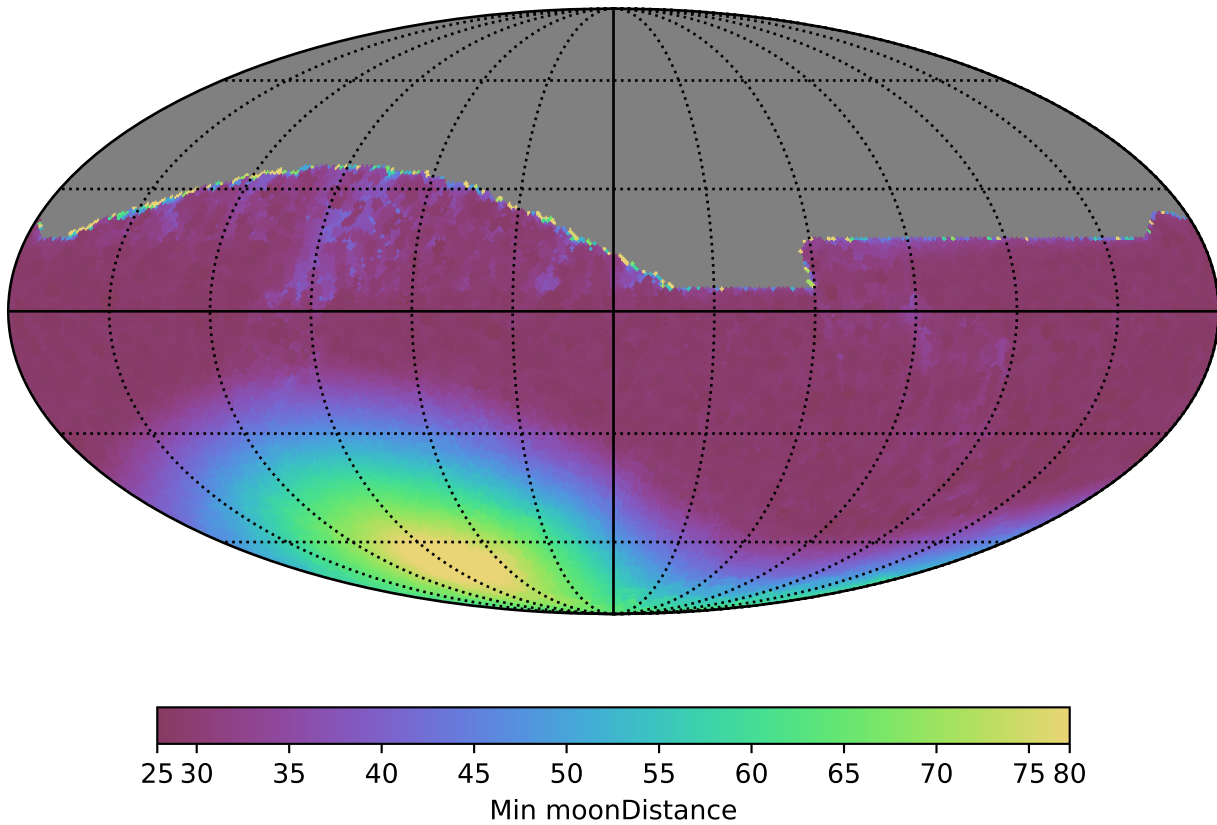
weather_cloudso10v3.4_10yrs All sky all bands: Min moonDistance
