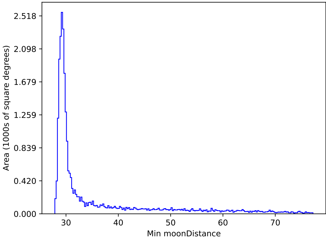
weather_cloudso10v3.4_10yrs All sky all bands: Min moonDistance
