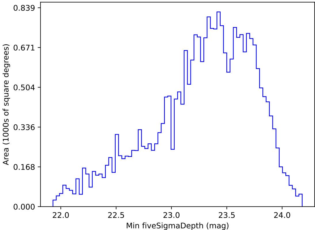
weather_cloudso10v3.4_10yrs Yr 1 r band: Min fiveSigmaDepth
