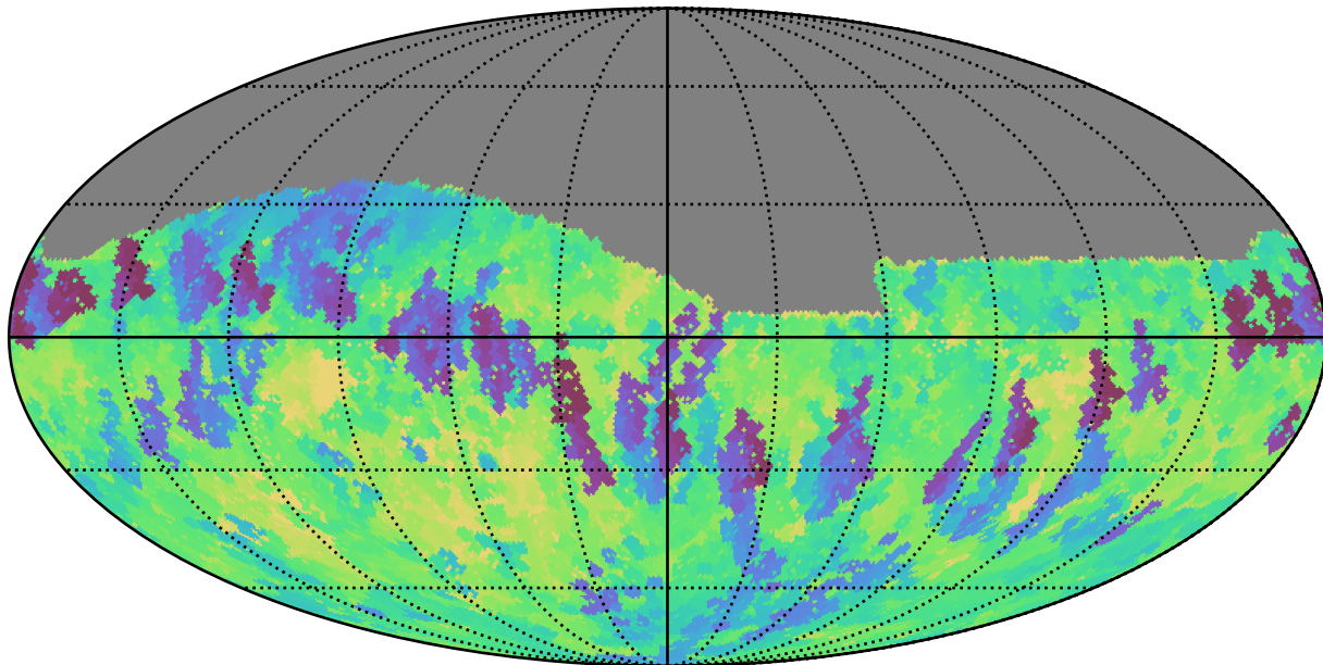
weather_cloudso10v3.4_10yrs Yr 1 i band: Min fiveSigmaDepth
