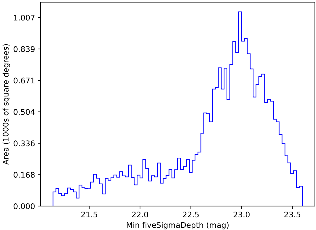
weather_cloudso10v3.4_10yrs Yr 1 i band: Min fiveSigmaDepth
