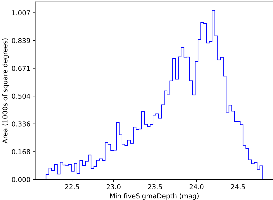
weather_cloudso10v3.4_10yrs Yr 1 g band: Min fiveSigmaDepth
