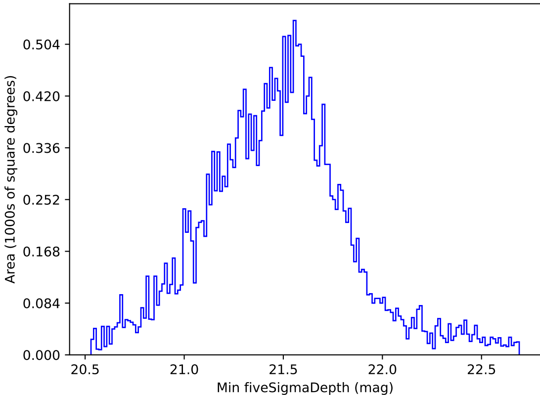
weather_cloudso10v3.4_10yrs Yr 1 all bands: Min fiveSigmaDepth
