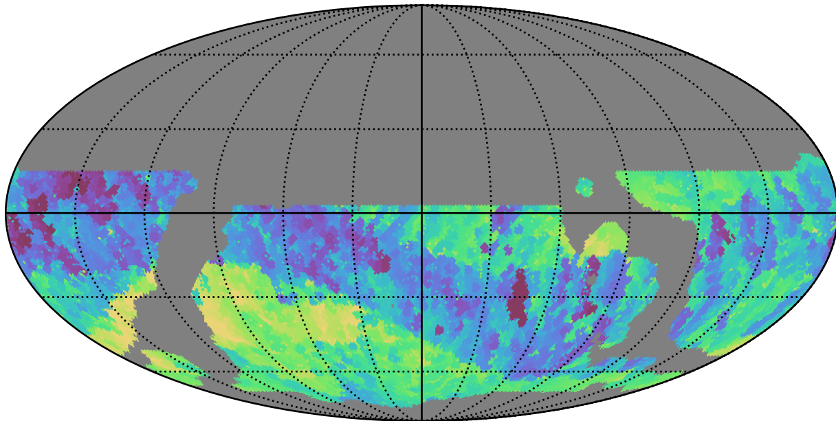
weather_cloudso10v3.4_10yrs WFD z band: Min fiveSigmaDepth
