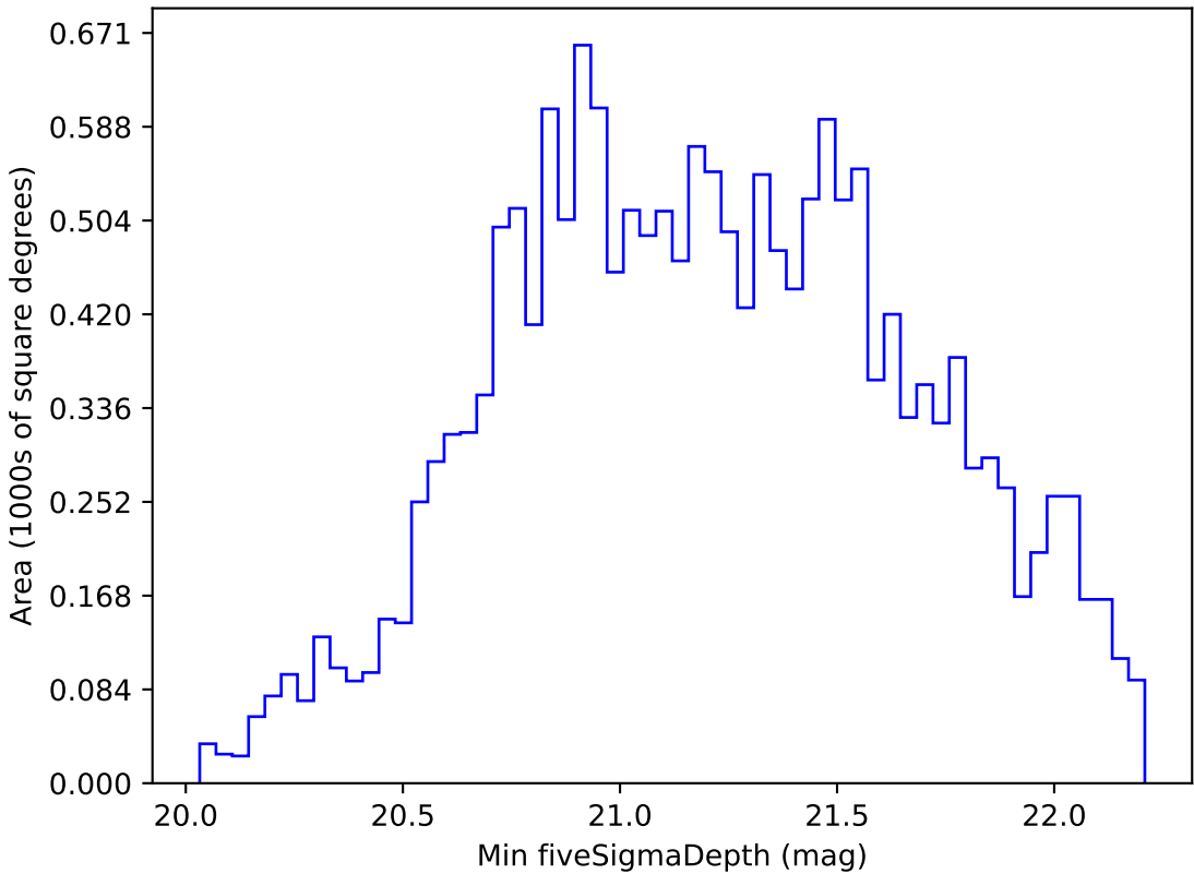
weather_cloudso10v3.4_10yrs WFD z band: Min fiveSigmaDepth
