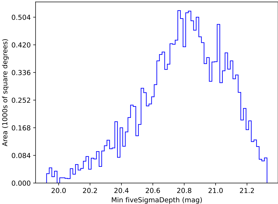
weather_cloudso10v3.4_10yrs WFD y band: Min fiveSigmaDepth
