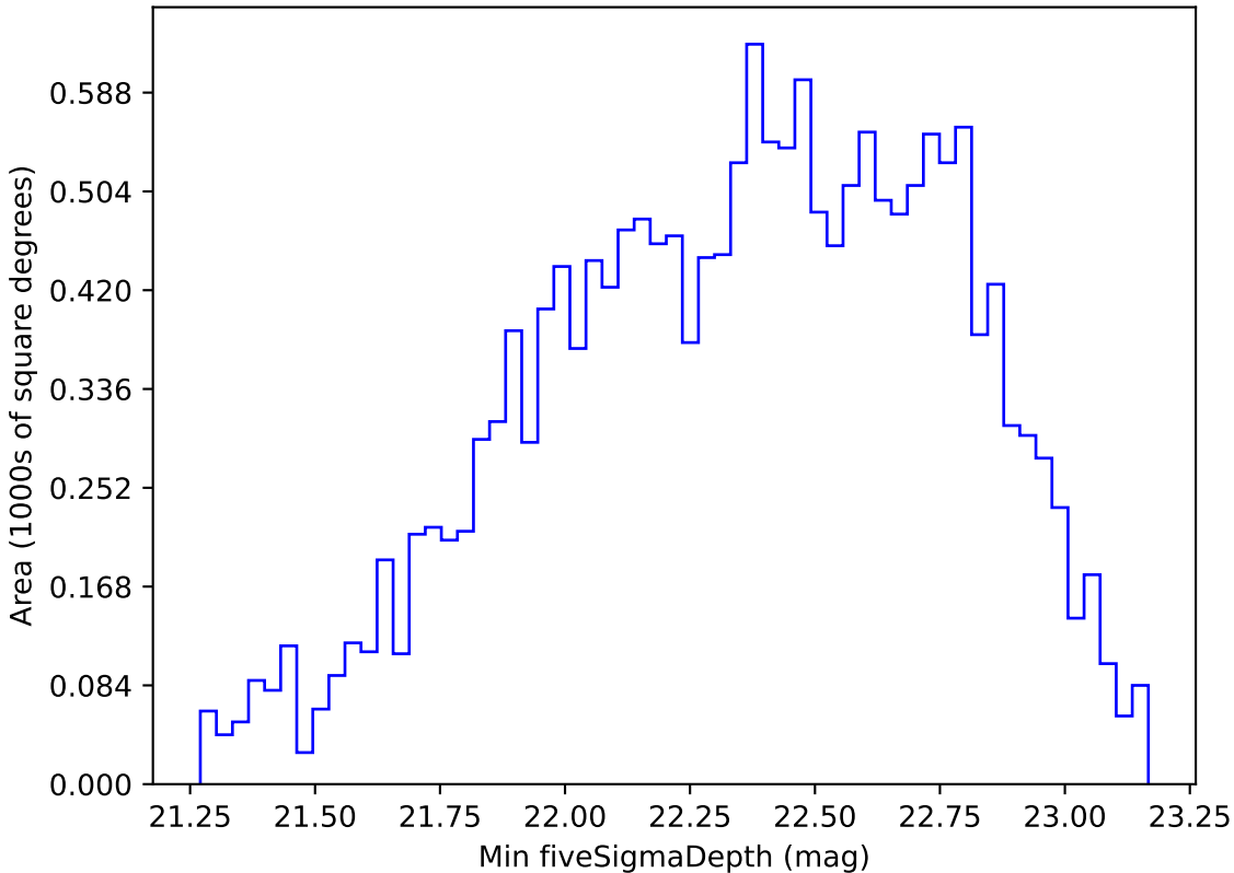
weather_cloudso10v3.4_10yrs WFD r band: Min fiveSigmaDepth
