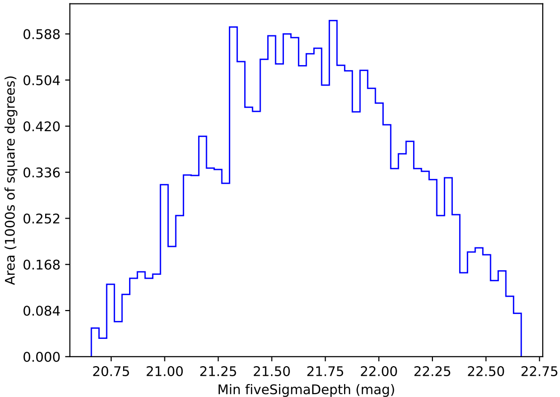
weather_cloudso10v3.4_10yrs WFD i band: Min fiveSigmaDepth
