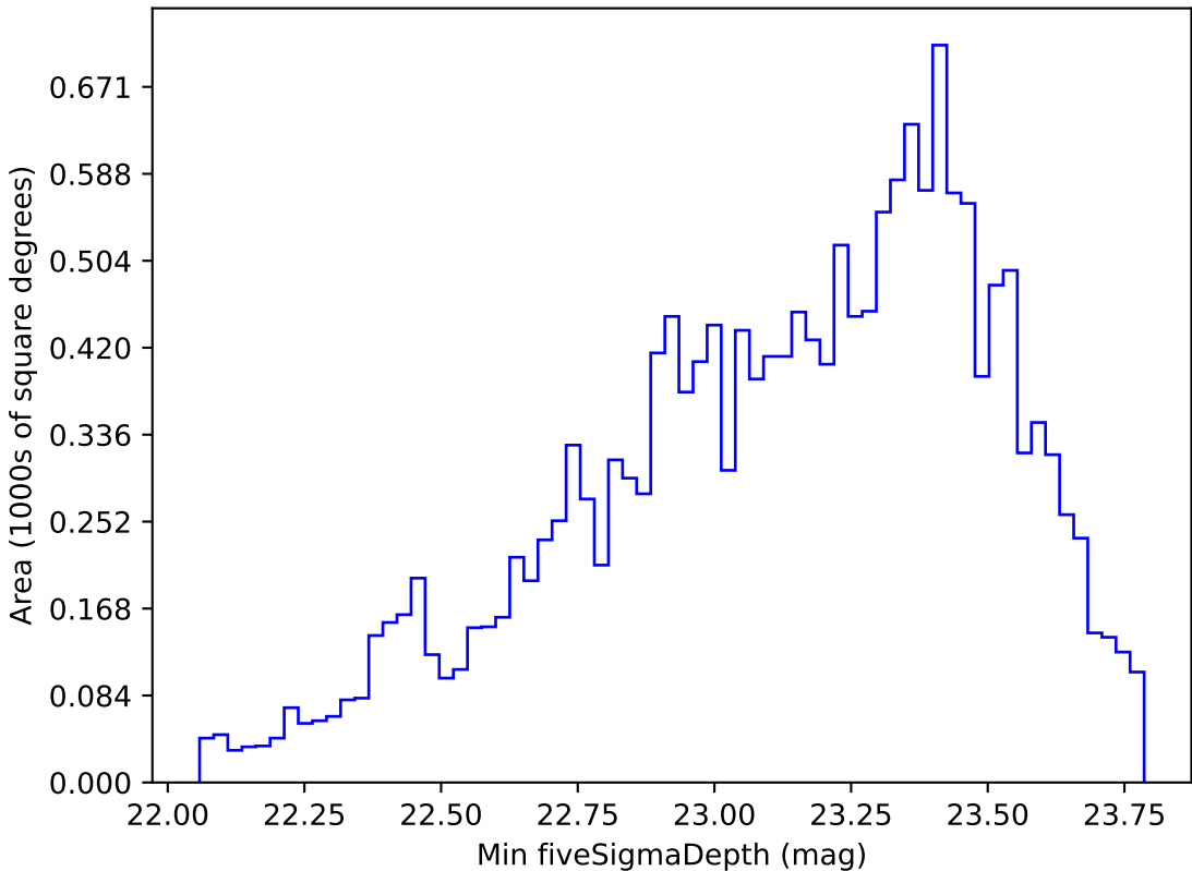
weather_cloudso10v3.4_10yrs WFD g band: Min fiveSigmaDepth
