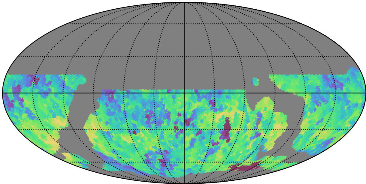
weather_cloudso10v3.4_10yrs WFD all bands: Min fiveSigmaDepth
