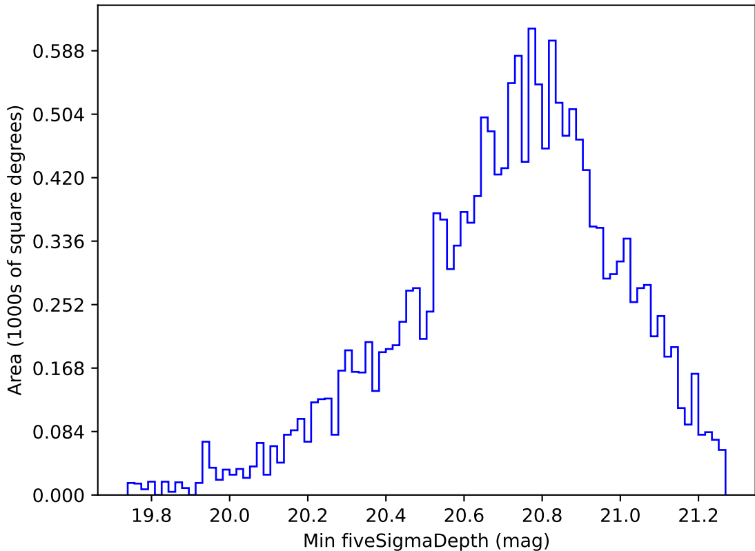
weather_cloudso10v3.4_10yrs WFD all bands: Min fiveSigmaDepth
