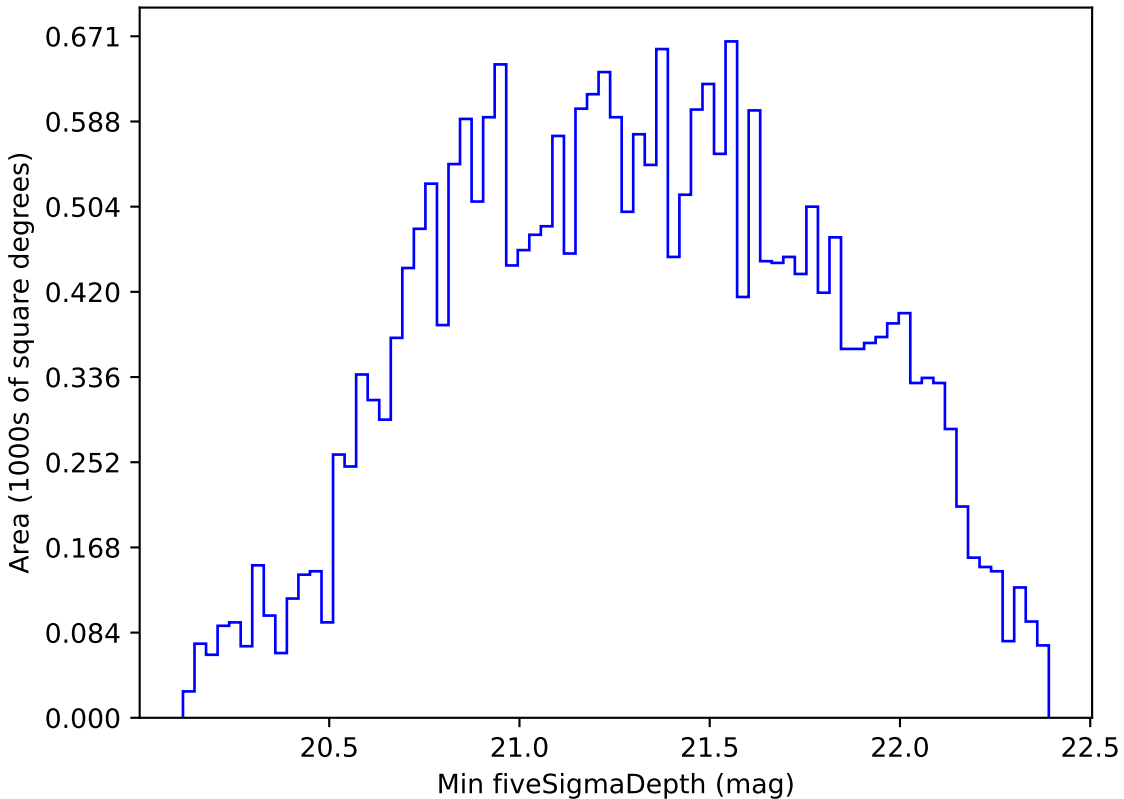
weather_cloudso10v3.4_10yrs All sky z band: Min fiveSigmaDepth
