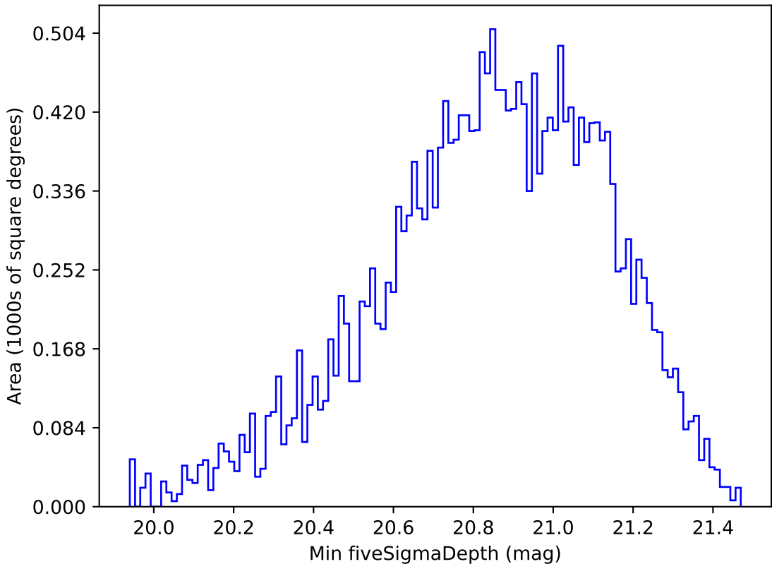
weather_cloudso10v3.4_10yrs All sky y band: Min fiveSigmaDepth
