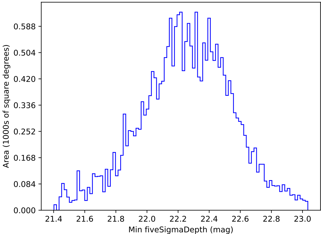
weather_cloudso10v3.4_10yrs All sky u band: Min fiveSigmaDepth
