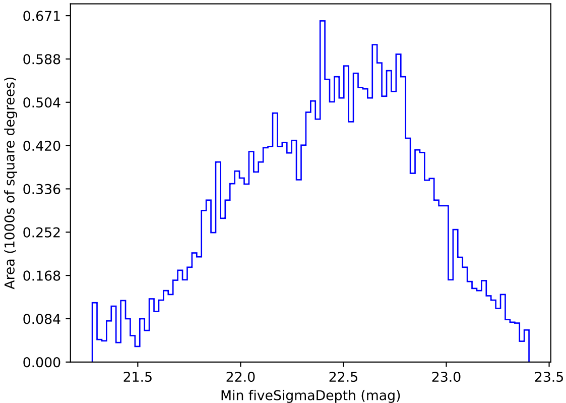
weather_cloudso10v3.4_10yrs All sky r band: Min fiveSigmaDepth
