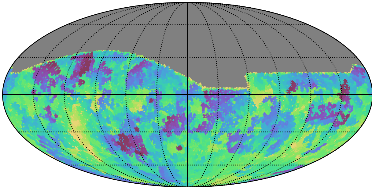
weather_cloudso10v3.4_10yrs All sky g band: Min fiveSigmaDepth
