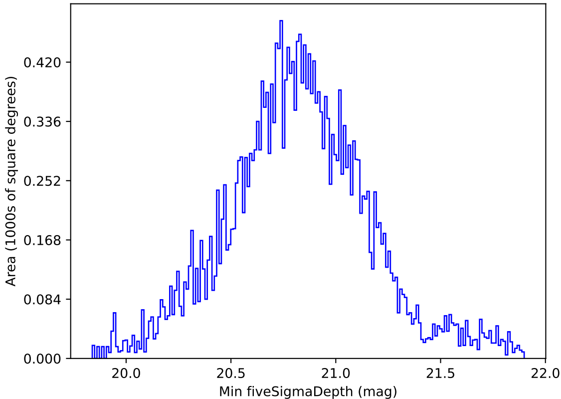
weather_cloudso10v3.4_10yrs All sky all bands: Min fiveSigmaDepth
