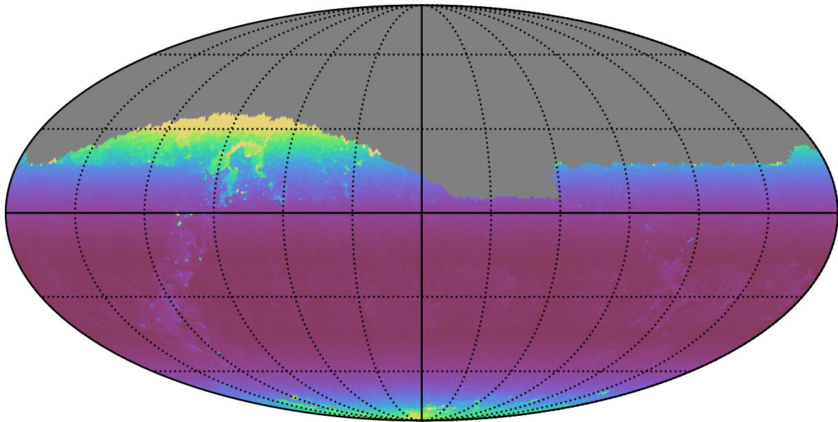
weather_cloudso10v3.4_10yrs Yr 1 z band: Min airmass
