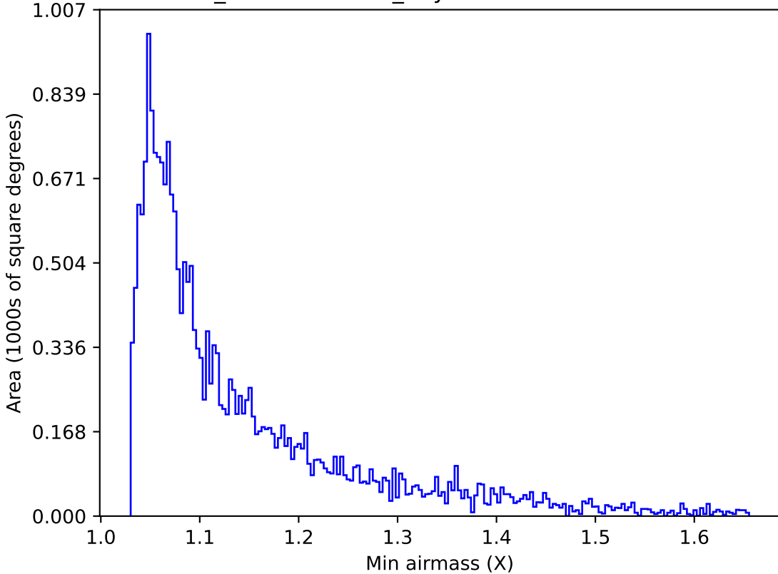
weather_cloudso10v3.4_10yrs Yr 1 u band: Min airmass
