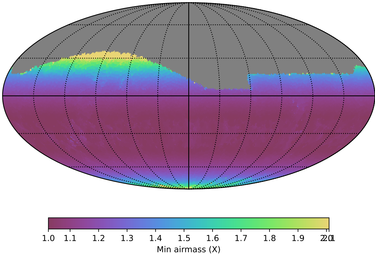
weather_cloudso10v3.4_10yrs Yr 1 r band: Min airmass
