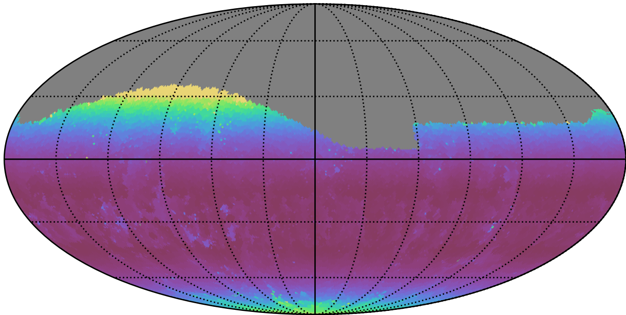
weather_cloudso10v3.4_10yrs Yr 1 g band: Min airmass
