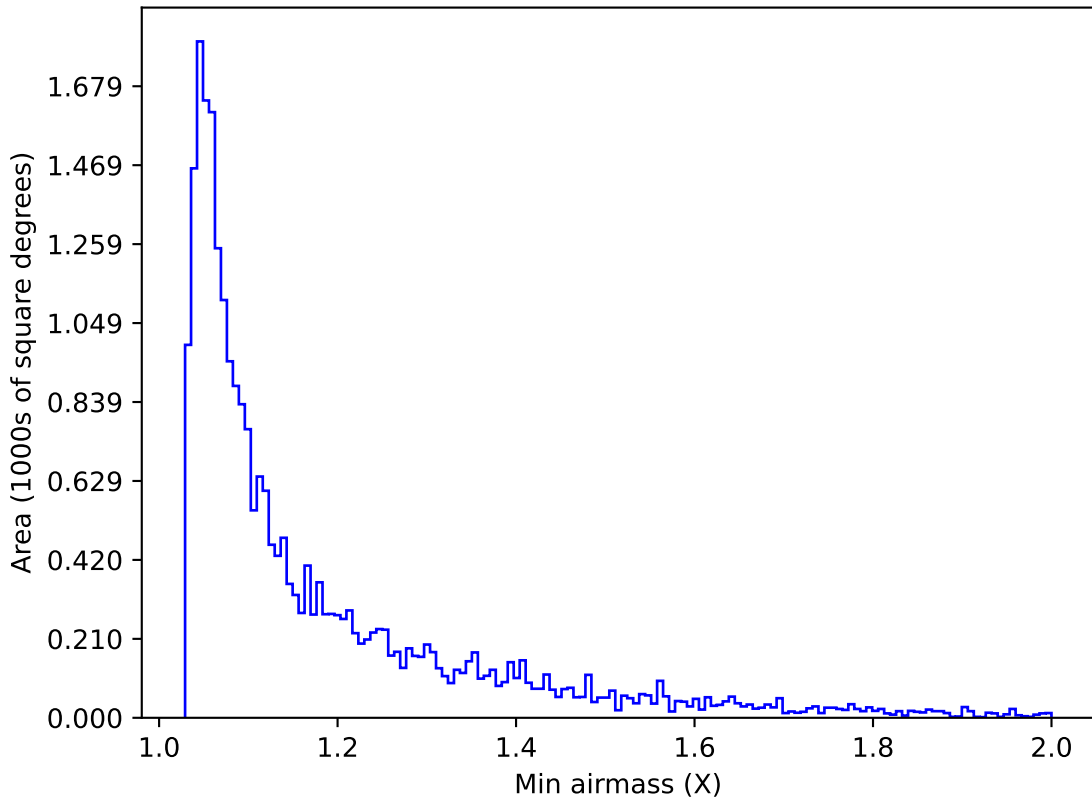
weather_cloudso10v3.4_10yrs Yr 1 g band: Min airmass
