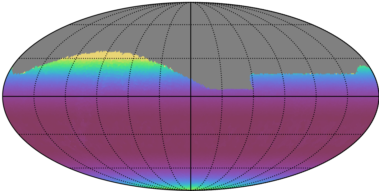
weather_cloudso10v3.4_10yrs Yr 1 all bands: Min airmass
