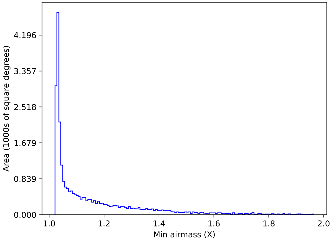
weather_cloudso10v3.4_10yrs Yr 1 all bands: Min airmass
