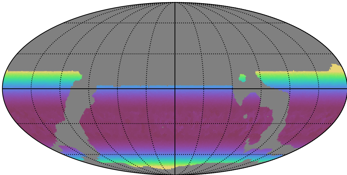
weather_cloudso10v3.4_10yrs WFD z band: Min airmass
