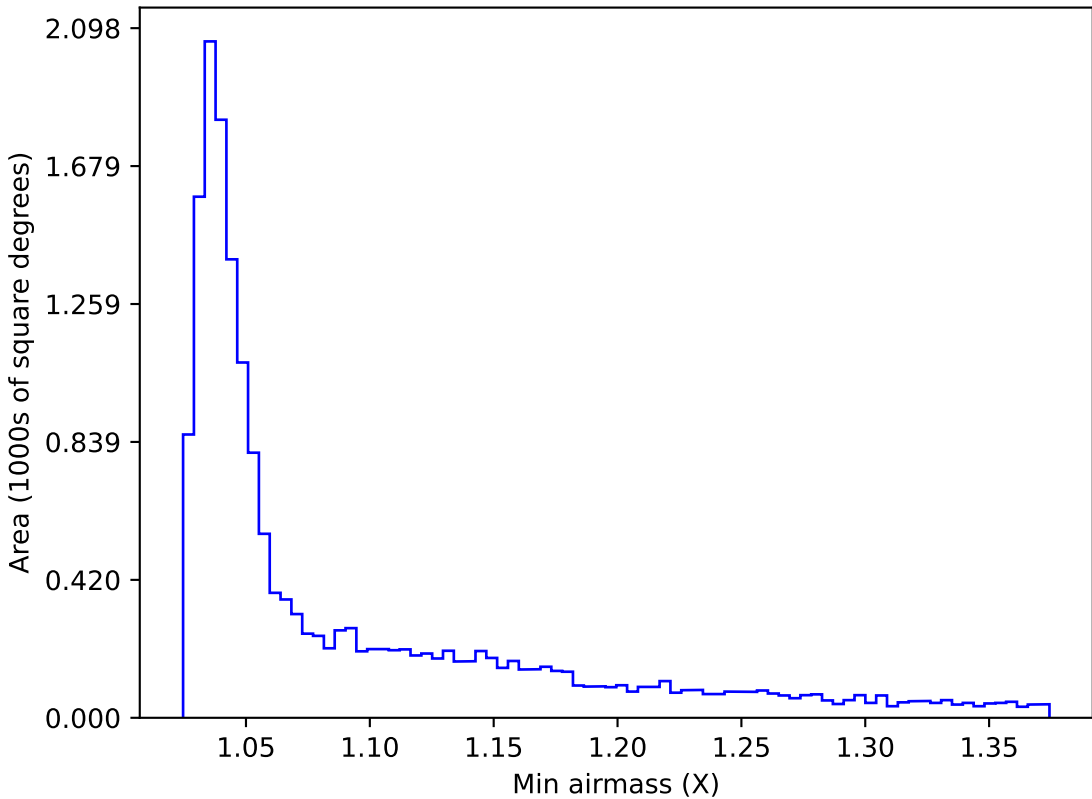
weather_cloudso10v3.4_10yrs WFD u band: Min airmass
