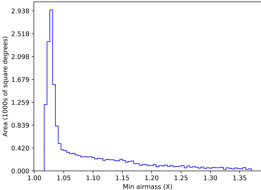
weather_cloudso10v3.4_10yrs WFD r band: Min airmass
