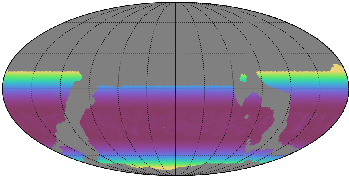
weather_cloudso10v3.4_10yrs WFD i band: Min airmass
