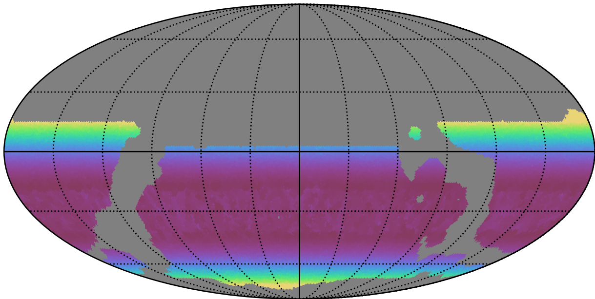
weather_cloudso10v3.4_10yrs WFD g band: Min airmass
