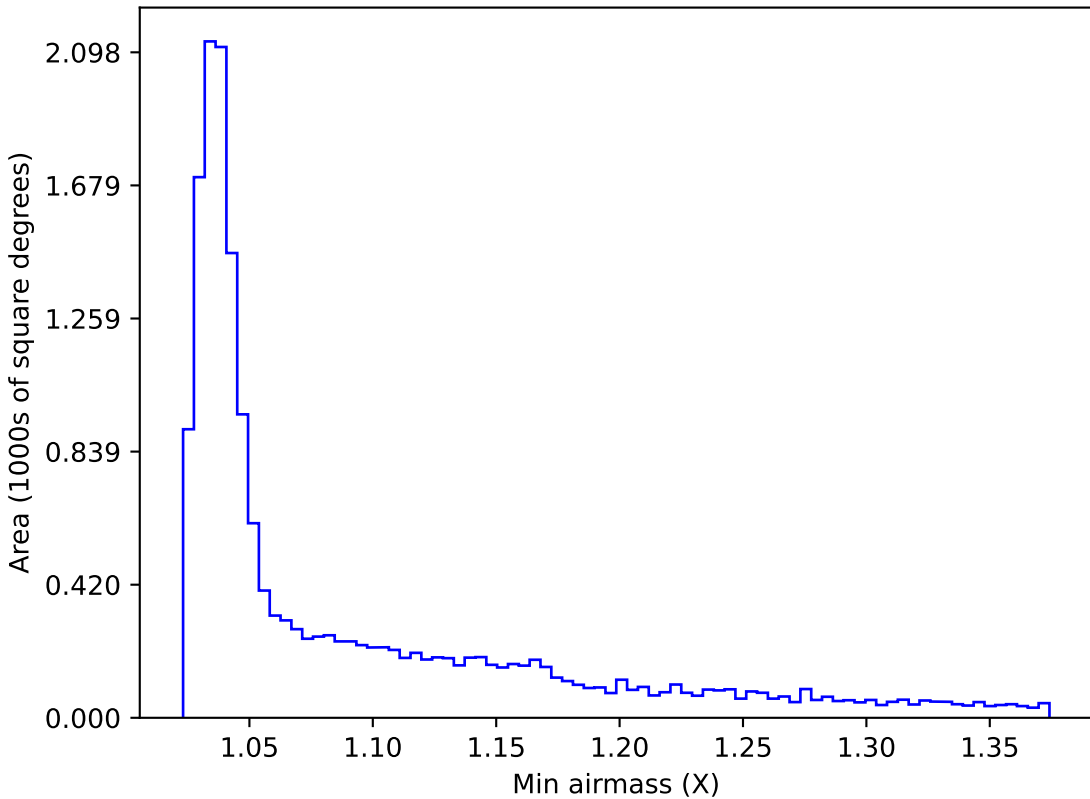
weather_cloudso10v3.4_10yrs WFD g band: Min airmass
