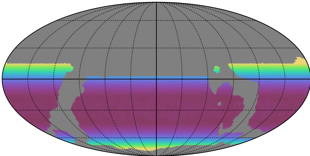
weather_cloudso10v3.4_10yrs WFD all bands: Min airmass
