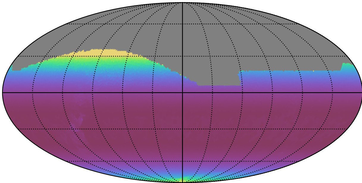
weather_cloudso10v3.4_10yrs All sky z band: Min airmass
