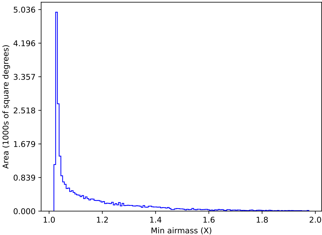
weather_cloudso10v3.4_10yrs All sky z band: Min airmass
