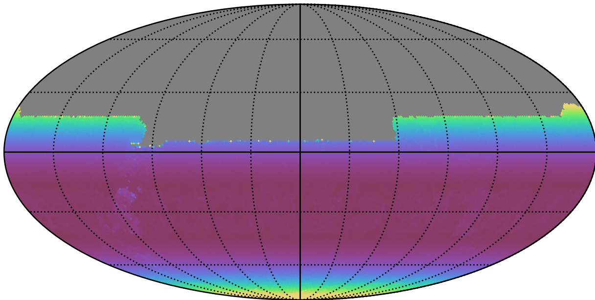
weather_cloudso10v3.4_10yrs All sky y band: Min airmass
