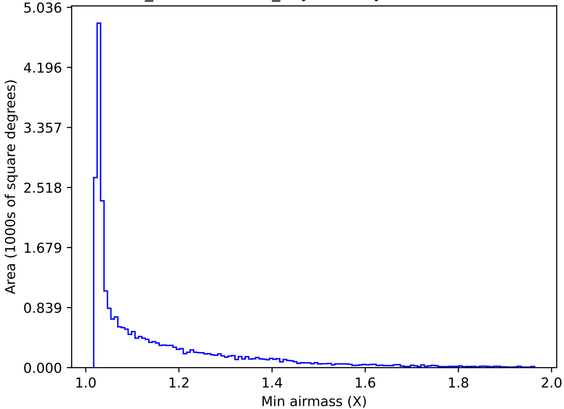
weather_cloudso10v3.4_10yrs All sky r band: Min airmass
