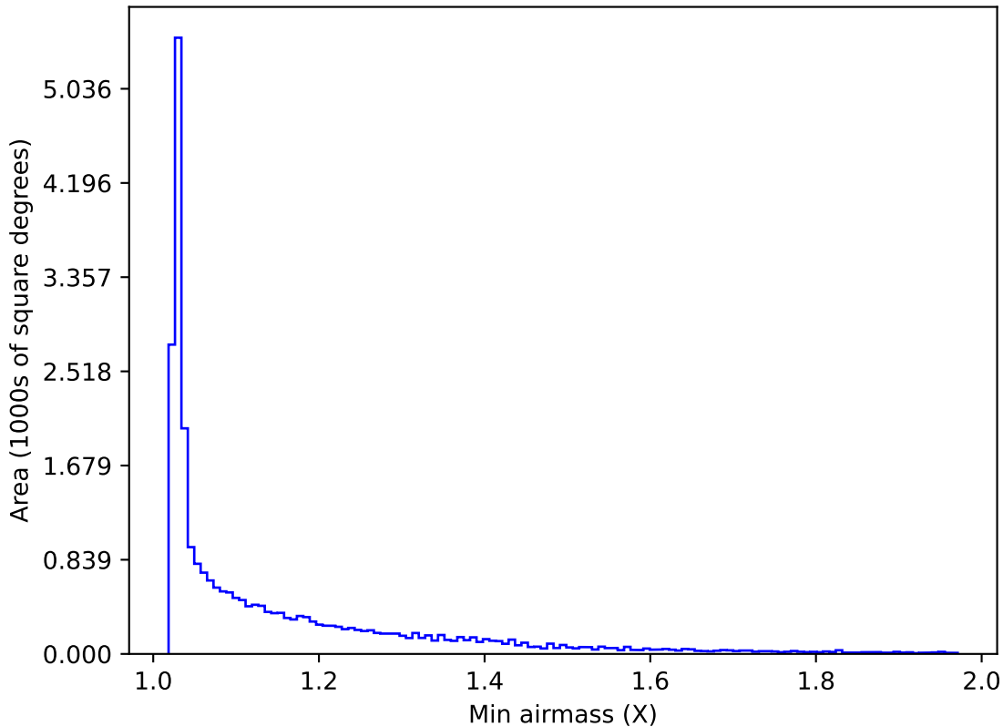
weather_cloudso10v3.4_10yrs All sky i band: Min airmass
