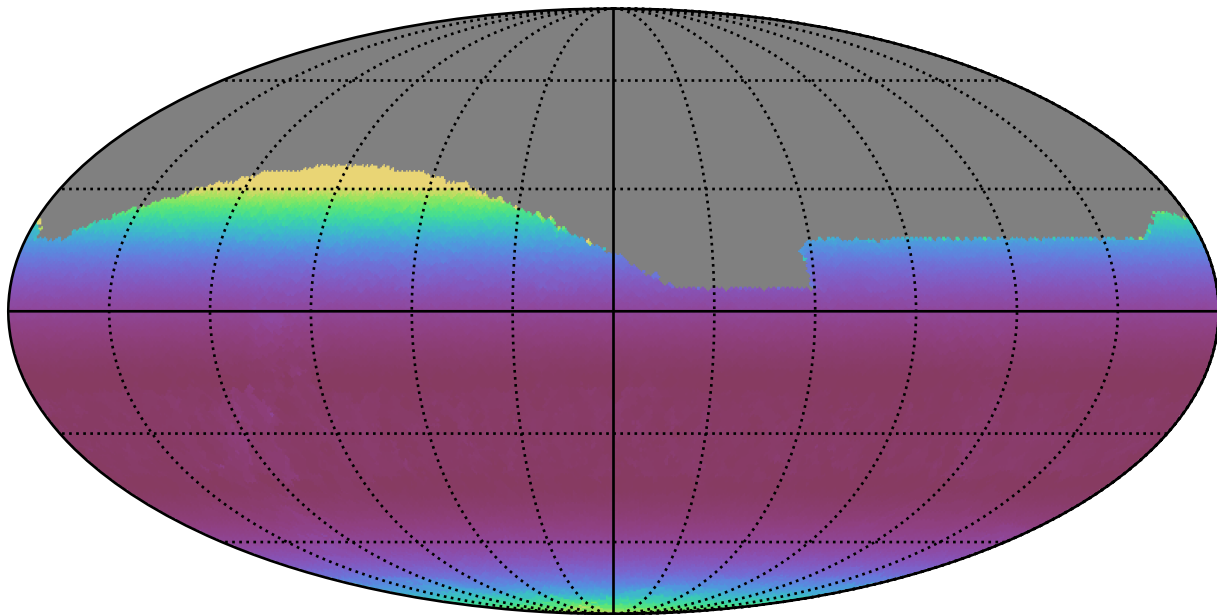
weather_cloudso10v3.4_10yrs All sky g band: Min airmass
